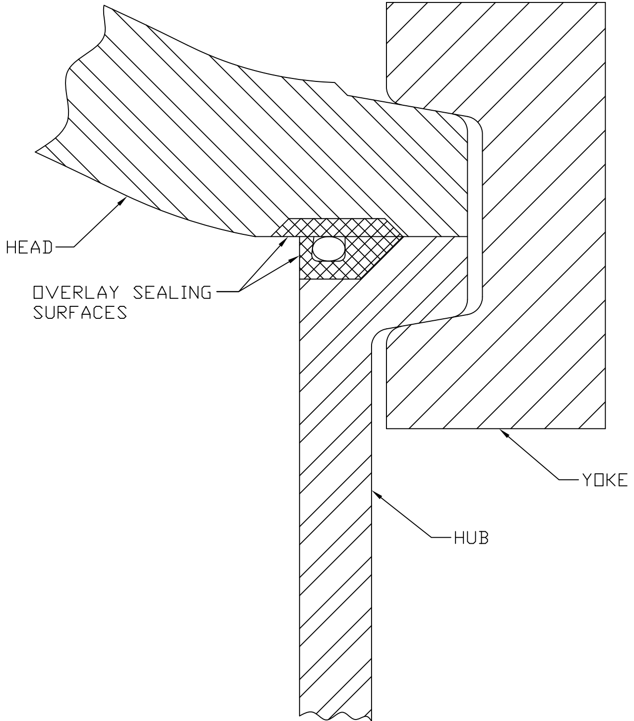
DOUBLE BOLT CLOSURE WITH CORROSION RESISTANT WELD OVERLAY
